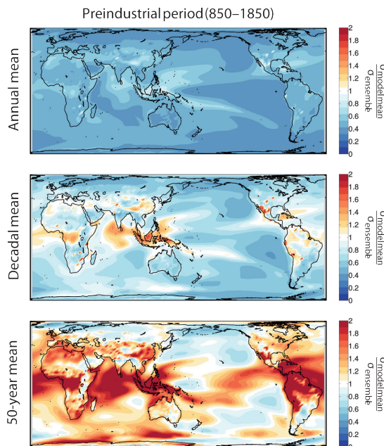
Figure 1: Ratio of the standard deviation of the ensemble mean of an ensemble of 10 simulations performed with CESM1 (Otto-Bliesner et al., 2016) over the mean standard deviation of the ensemble members around this ensemble mean, for the 2-meter air temperature. The standard deviations are computed over the period C.E. 850-1850 for (top panel) annual mean values (middle panel) decadal-means and (bottom panel) 50-year means. The ensemble mean is representative of the forced response while the range of the ensemble around this ensemble mean provides an estimate of the internal variability as simulated by the model.
